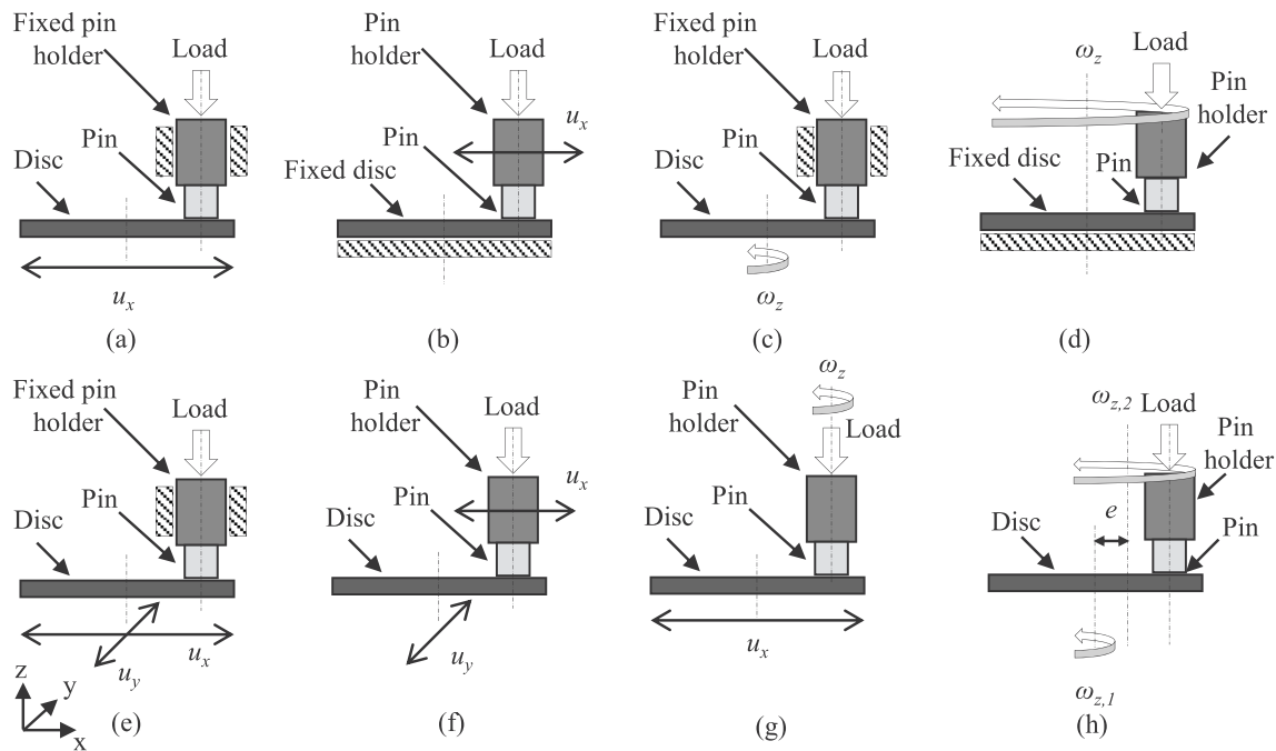
Fig. 1. Schematic of eight different PoD wear measurement configurations used in the context of prosthetic hip implants, showing the relative motion between the pin and the disc. u_x and u_y are the velocity magnitude in the x - and y -directions, and \omega_z is angular velocity about the z -direction.
