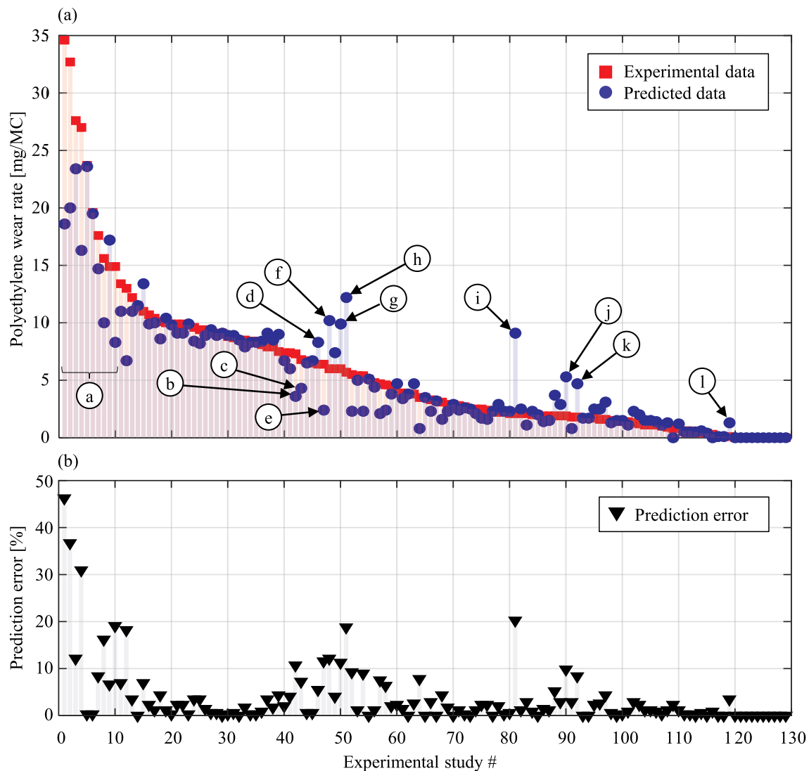
Fig. 3. Polyethylene wear rate for all experimental studies considered in our dataset ranked in descending order, (a) showing the experimental results documented in the literature (red square markers) and the corresponding predicted results using the data-driven model based on the KNN method (blue circle markers), and (b) showing the prediction error for the corresponding experimental study (black triangle markers). (For interpretation of the references to colour in this figure legend, the reader is referred to the Web version of this article.)
