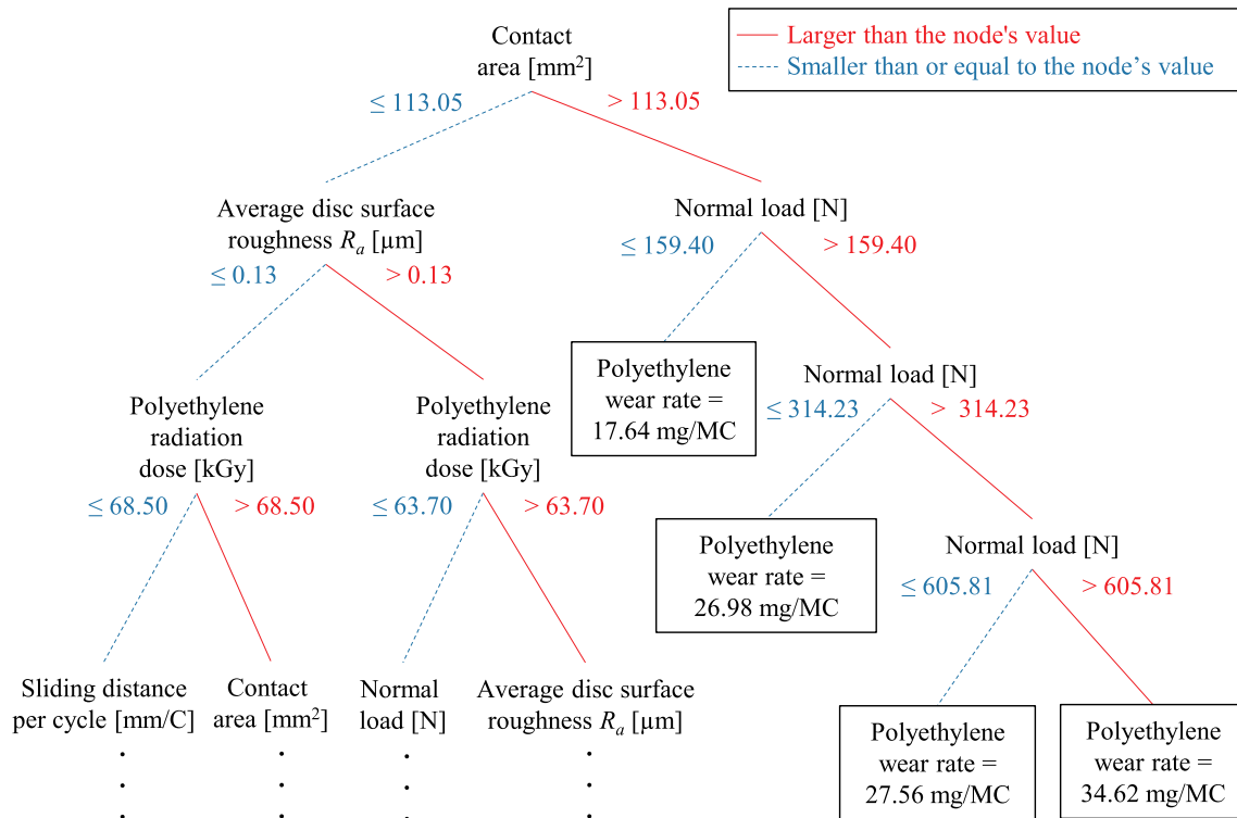
Fig. 4. First seven nodes of the CART model of the dataset considered in this work, showing how the attributes break down into a decision tree, ultimately predicting the target attribute and providing an interpretable model that relates the attributes (input) to the target attribute (output).
