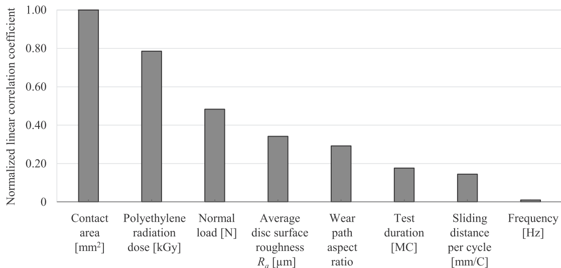
Fig. 2. Normalized linear correlation coefficient of each input attribute with the polyethylene wear rate (target attribute).
