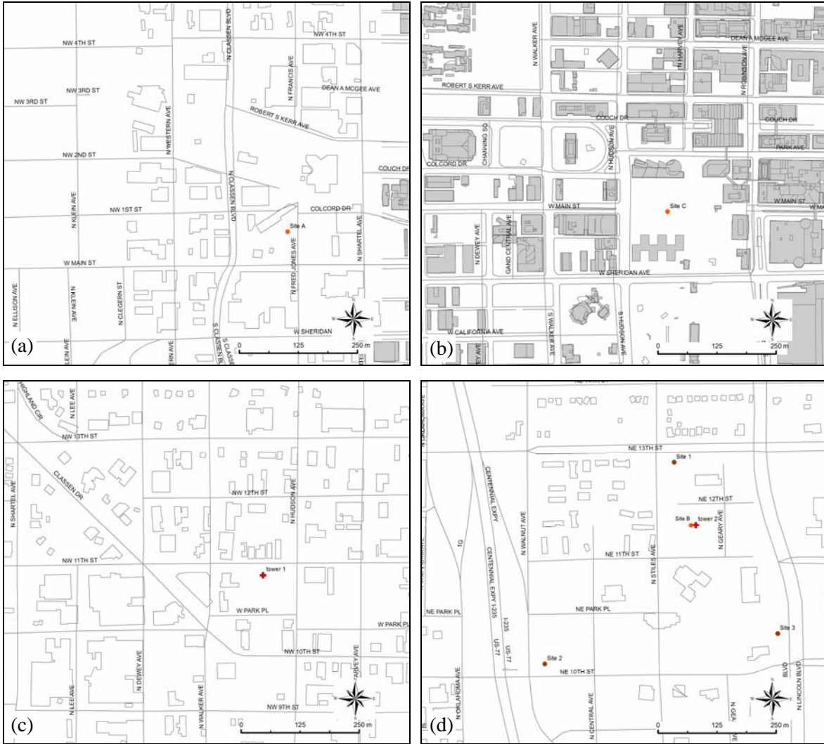
Figure A.14. ATDD Instrument Locations at (a) Energy Flux Site A, (b) Energy Flux Site C, (c) Sonic Tower 1, and (d) Energy Flux Site B and Micro-barograph Pressure Sites 1 Through 3
