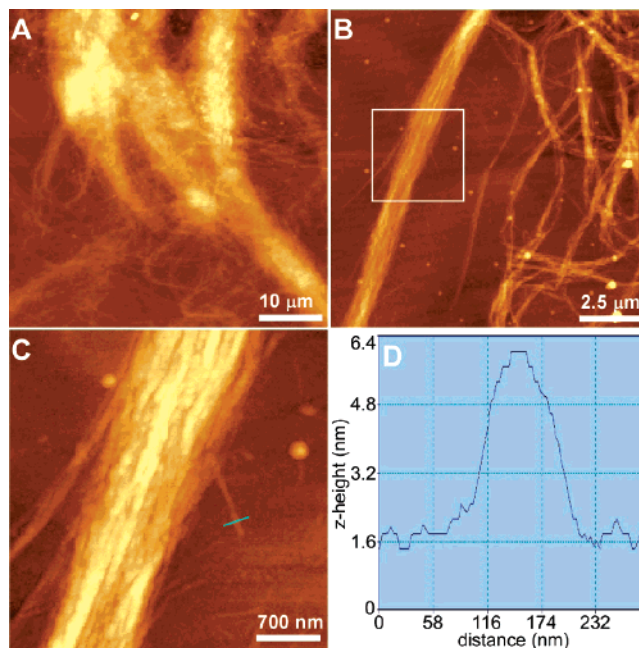
Figure 1. AFM images of the gel of 1 spin-cast and dried on glass: (A) large-area image showing the fibril piles; (B) different sizes of fibril bundles; (C) a zoomed-in image over a bundle marked in B; (D) z -height line scan profile over a single fiber marked in C. The total z -height ranges for A–C are 390, 49, and 28 nm, respectively.
