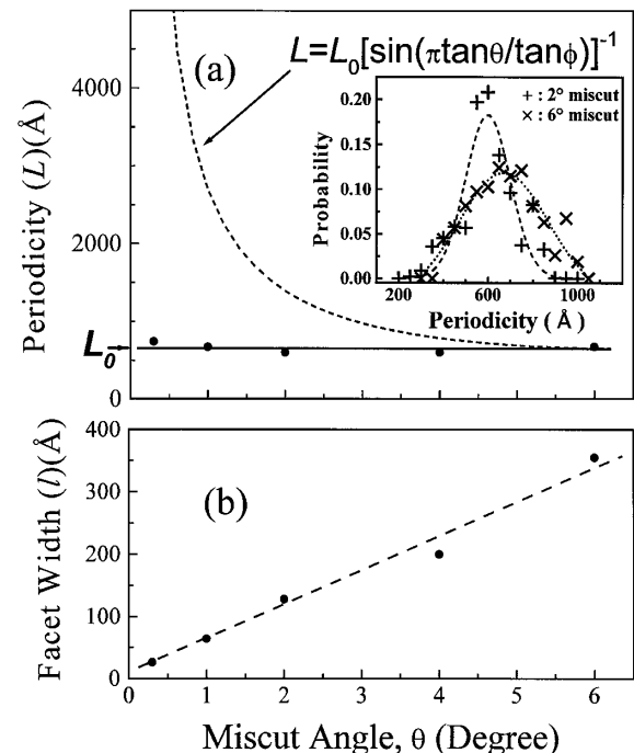
FIG. 2. Dependence of faceting periodicity and facet width on a miscut angle. (a) All ordered patterns adopt a universal periodicity of \sim 635 \text{ \AA} , independent of miscut angle. Values (dots) for different miscuts are obtained from the peak positions of Gaussian fits to the measured data, as shown in the inset for 2^\circ and 6^\circ samples. The dashed line shows the dependence of periodicity on a miscut angle if a one-stage faceting transition had occurred. (b) The facet width increases linearly with increasing miscut angle. The straight line is a least-squares fit to the data (dots).
