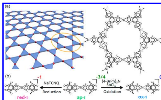
Figure 1. (a) Illustration of the chemical structure of the nickel bis(dithiolene) complex nanosheet. 1 corresponds to the stacked nanosheet. (b) Schematic illustration on redox control in 1 .
