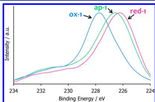
Figure 2. S 2s peak for the XPS of 1 (blue: ox-1 ; green: ap-1 ; red: red-1 ).
