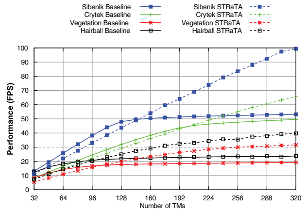
Figure 7: Performance on a selection of benchmark scenes with varying number of TMs. Each TM has 32 cores. Performance plateaus due to DRAM overutilization.
