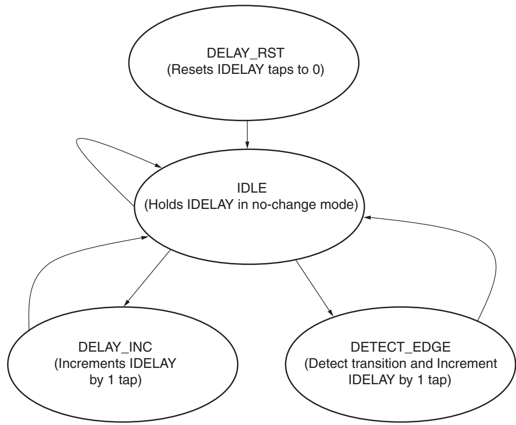
Figure 3: Strobe Edge Detection State Diagram
