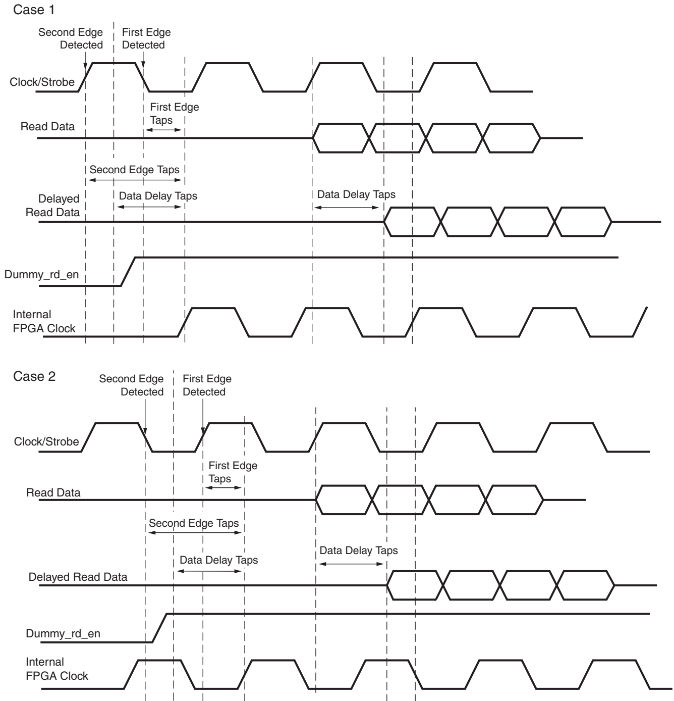
Figure 1: Case 1 and Case 2 - Clock/Strobe Center to Internal FPGA Clock Phase Detection
